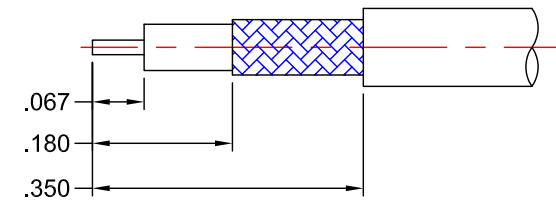
RECOMMENDED STRIPPING DIMENSIONS
